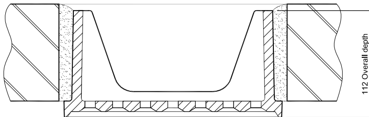
Sectional Plan
