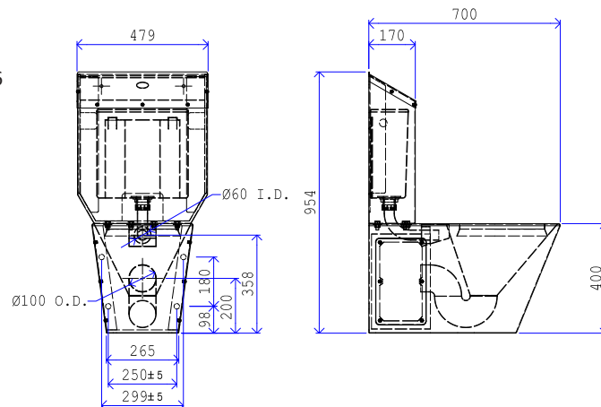
CSL0907DP Disabled Pneumatic Operation
